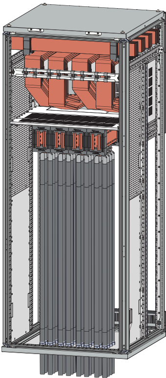
Cable Connections from Bottom of the Module
