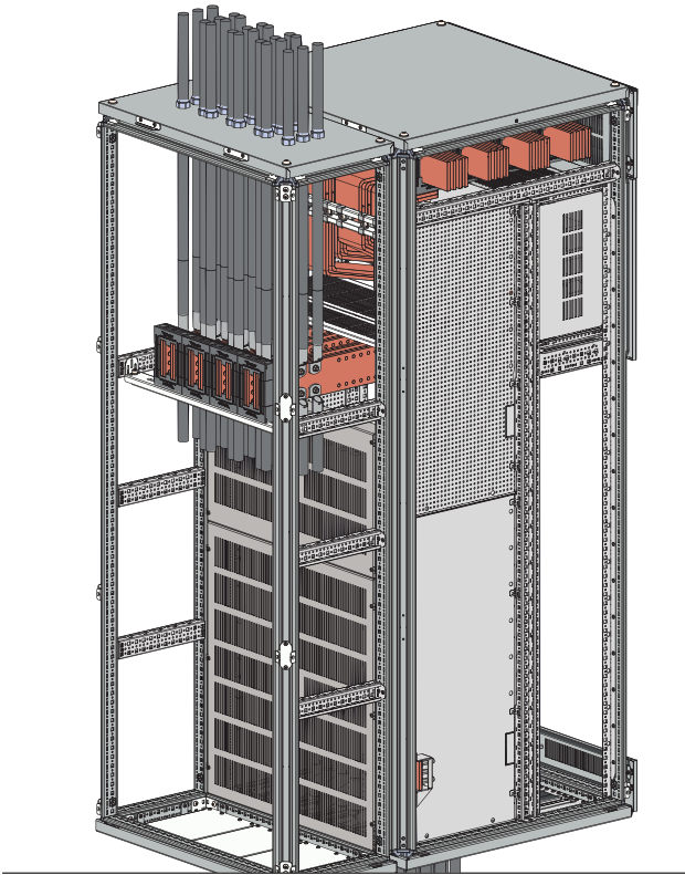
Cable Connections from Top via the Rear Cable Module
