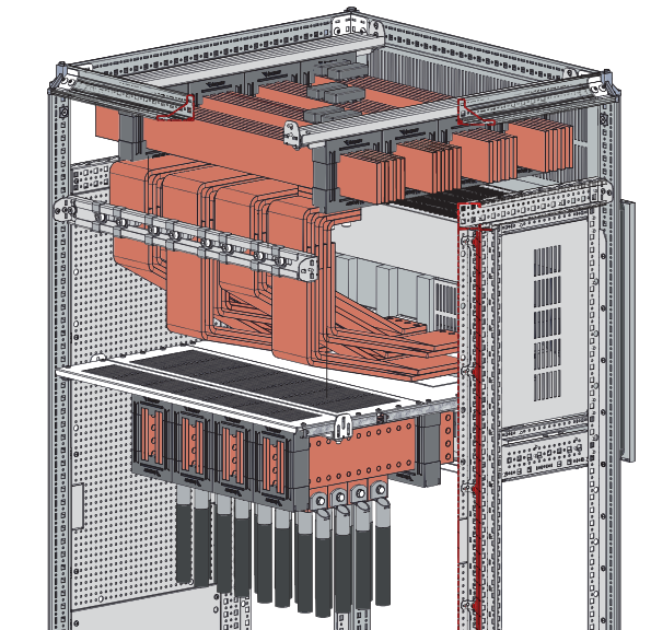
Conductor Connections from ACB Output to Cable Bar in the Module
