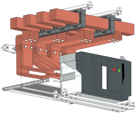
Conductor Connections from Main Busbar to ACB Input
