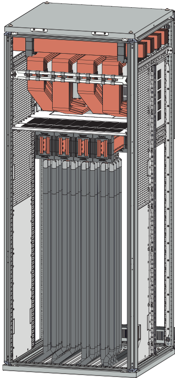
Cable Connections from Bottom of the Module (Foam Entry)
